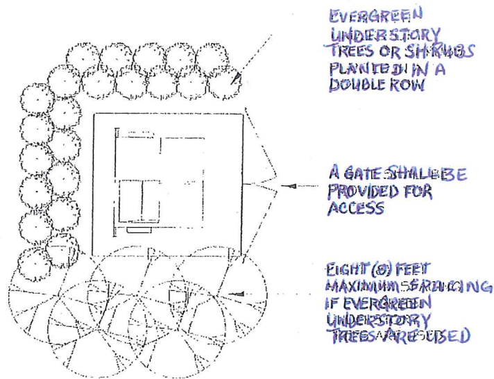
SCREENING BY USE OF EVERGREEN UNDERSTORY TREES AND SHRUBS
